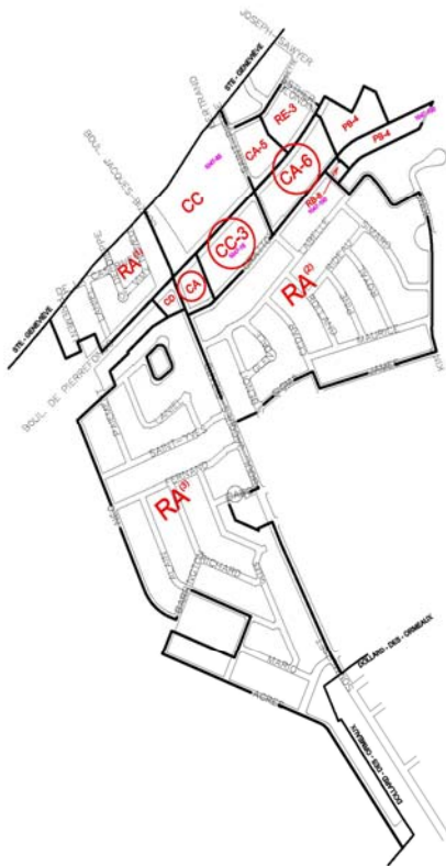
EXISTING ZONING
